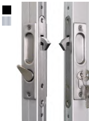
Flush Double Indent Handle with Key Lock
