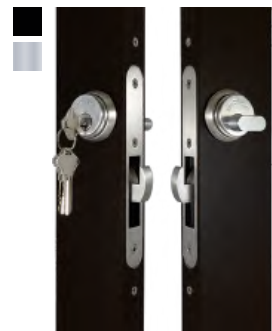
Latch Mechanism with 1" Mortise Key Cylinder and Thumbturn for Sliders
